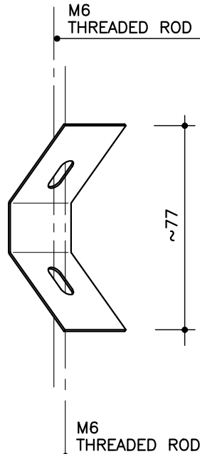
No. 70A SPRING CLIP
