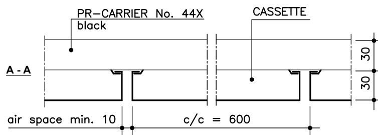
INSTALLATION WITH AIR SPACE AROUND THE CASSETTES
