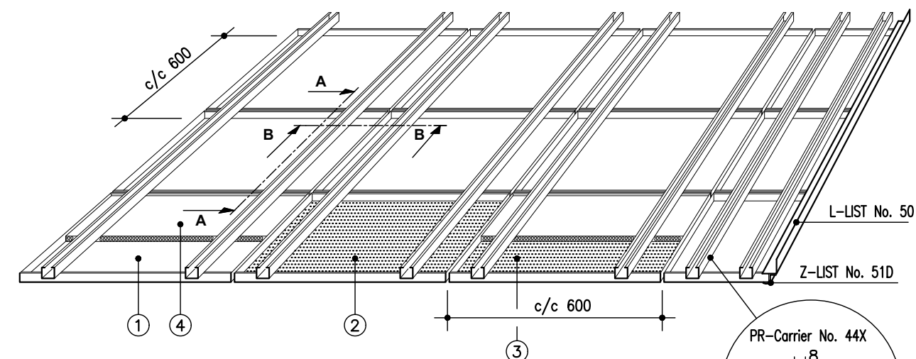
INSTALLATION WITH AIR SPACE AROUND THE CASSETTES
