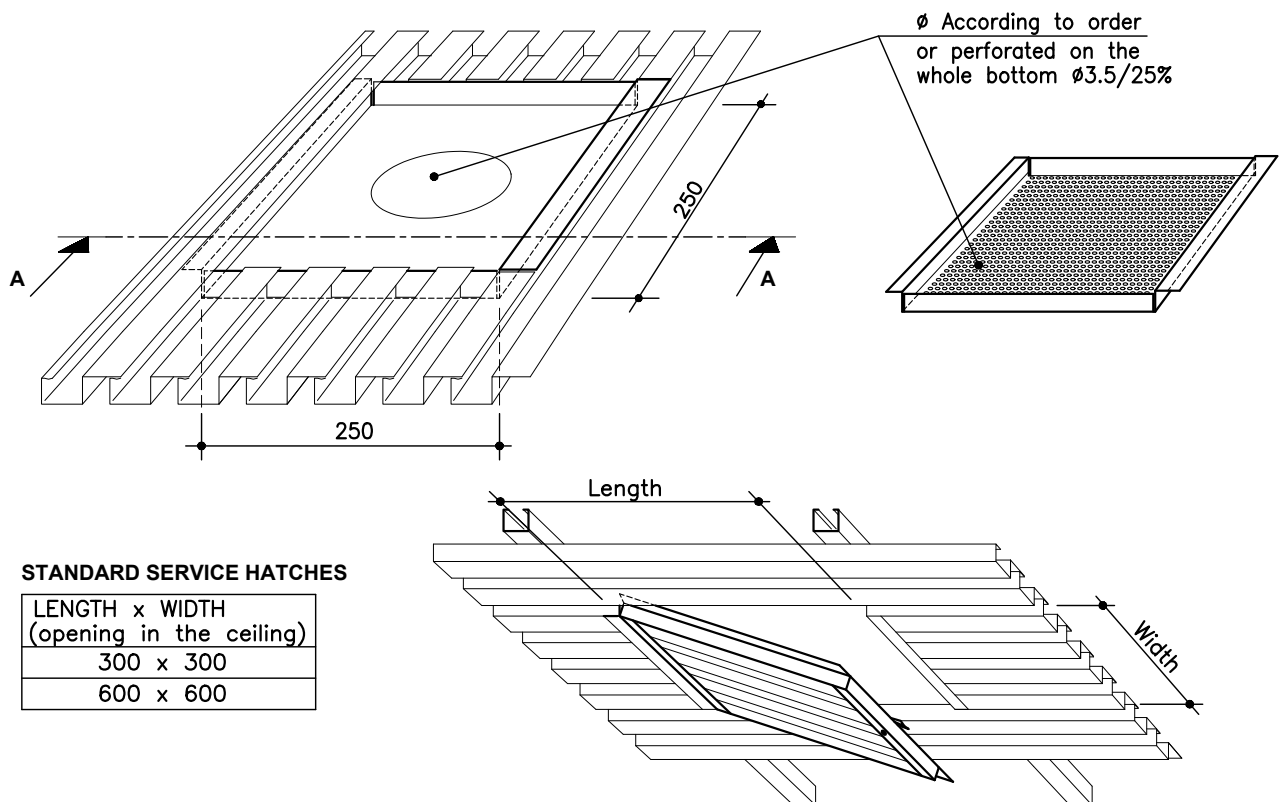
LOUDSPEAKER OR DOWNLIGHT PANEL
