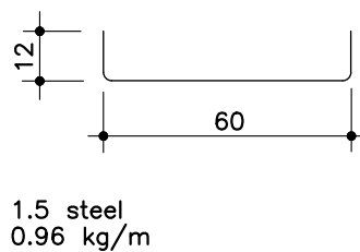
No. 55 SUPPORT PROFILE
