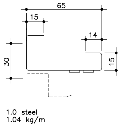
No. 54 SPRING-T-CARRIER
