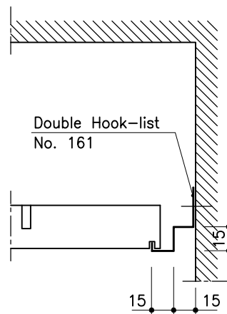
Fixed assembling
