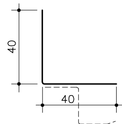
No. 50 L-LIST 40x40
