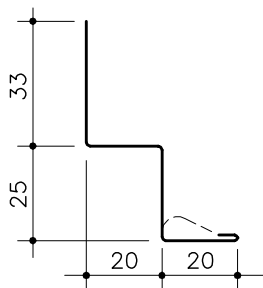
No. 31 DOUBLE-L-LIST WITH TONGUE
