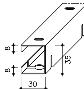
CARRIER WITH SCORES, No. 119
