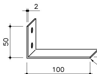
FASTENER TYPE 2
