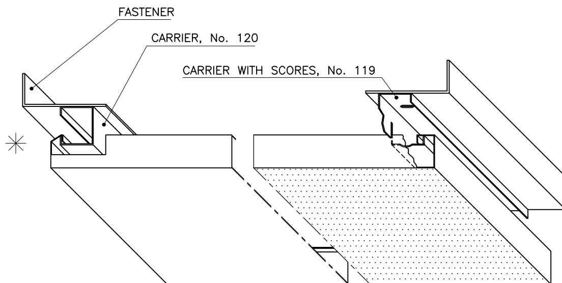
FASTENER TYPE 1, No. 121
