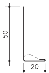
No. 34 L-LIST WITH TONGUE
