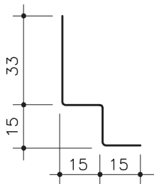
No. 30 DOUBLE-L-LIST
