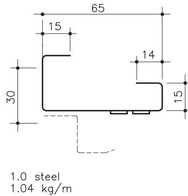
No. 54 SPRING-T-CARRIER
