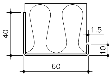
No. 168A J-LIST 1.5 Fe, stone wool 50 mm Density 110 kg/m 3
