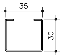
No. 90. CARRIER 1.0 Fe
