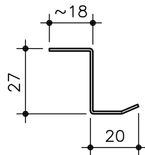
No. 51c. Z-LIST 1.0 Fe
