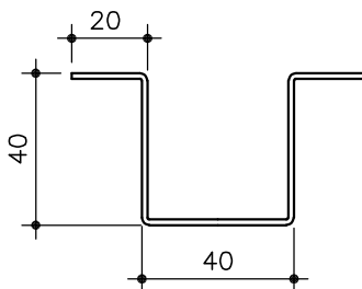
No. 166. CARRIER 1.5 Fe
