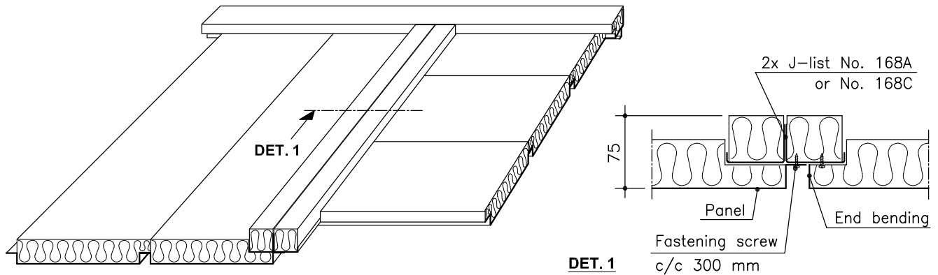
No. 90. CARRIER 1.0 Fe
