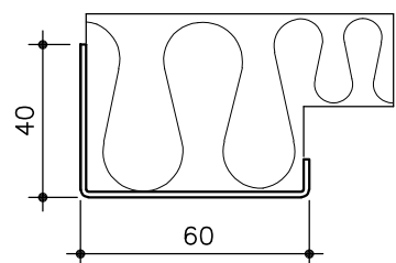
No. 168C J-LIST 1.5 Fe, special stone wool 50 mm Density 110 kg/m 3
