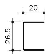
No. 53C+ U-INSERT LIST 0.6 Fe
