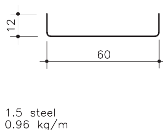
No. 55 SUPPORT PROFILE
