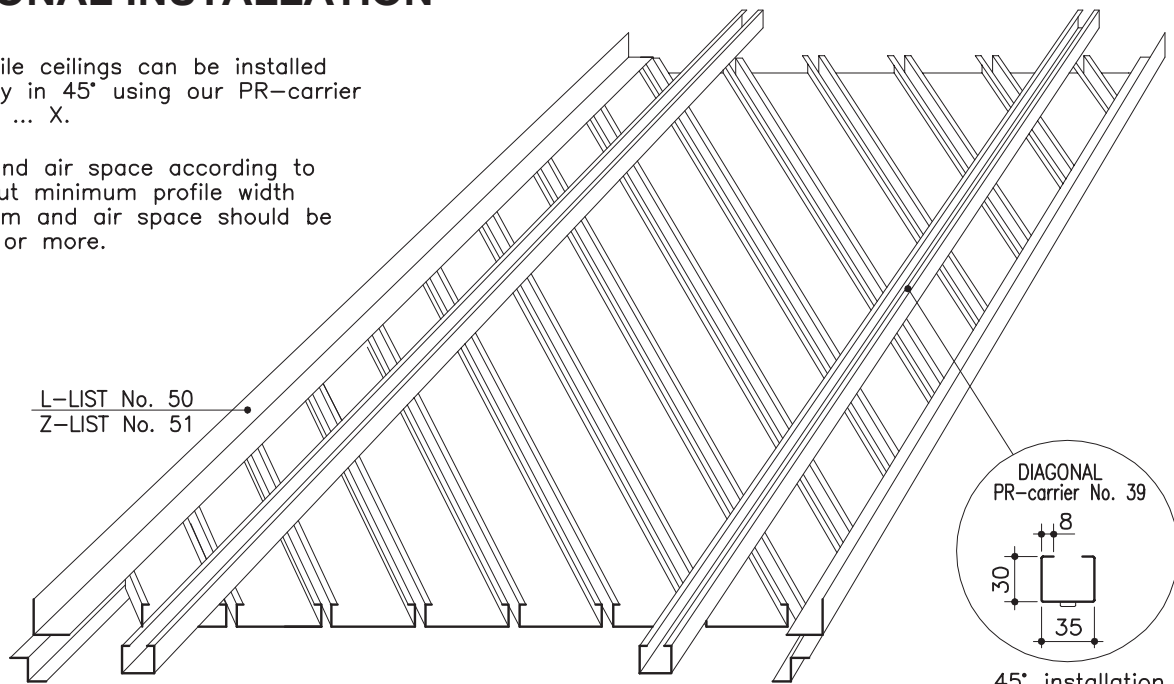
45° installation
