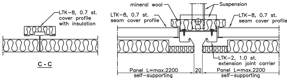
Ceiling extension joint If the panel is longer than 2200mm
